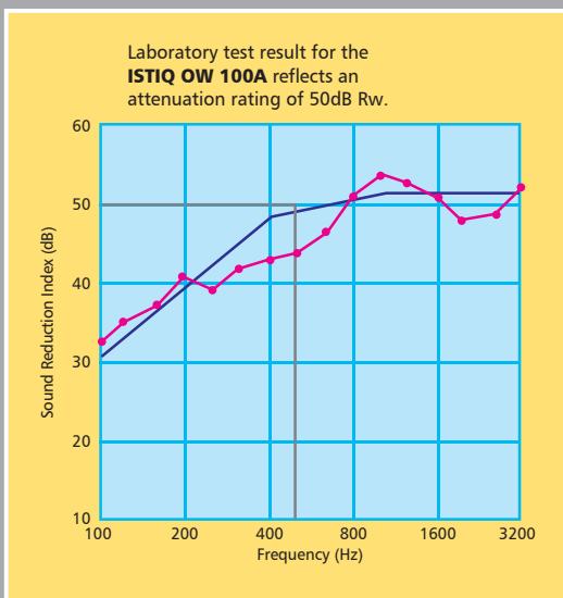
Fig. 1: Acoustic Performance
