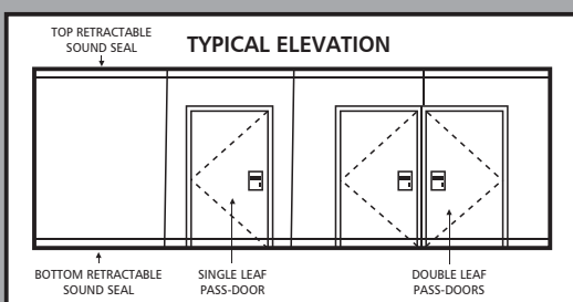
Fig. 2: Pass Doors
