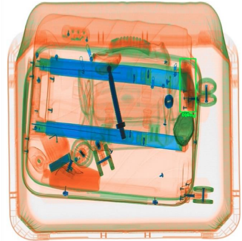
Explosive test piece in paste form.
