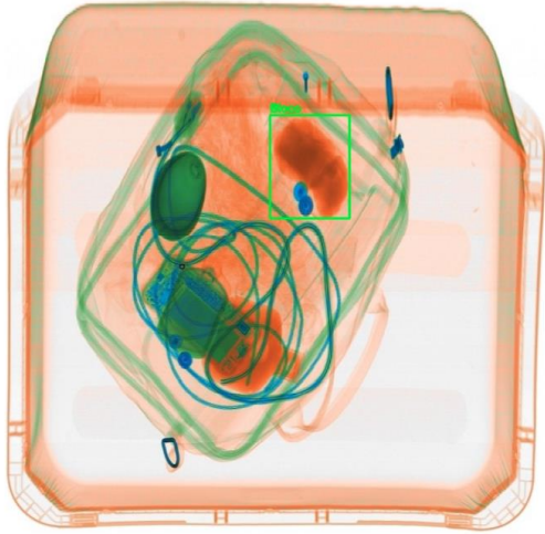
Block-shaped explosive test piece.
