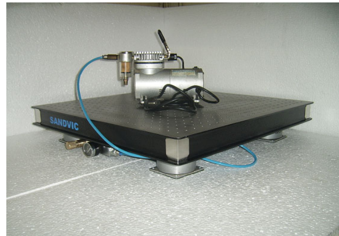
Desktop Vibration Isolation Module
